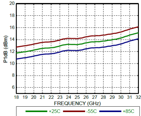
Output Power P_{1dB}
