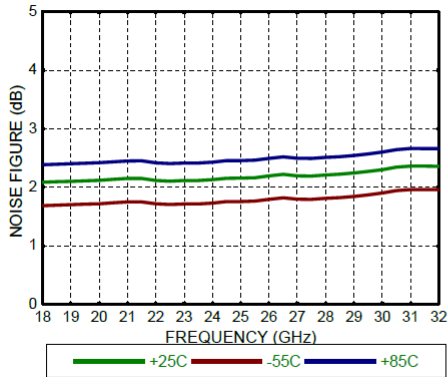
Noise Figure
