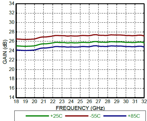
Gain
