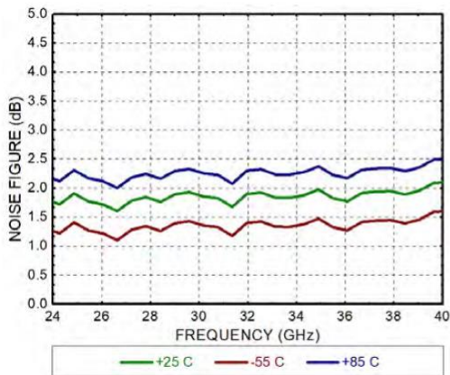
Noise Figure
