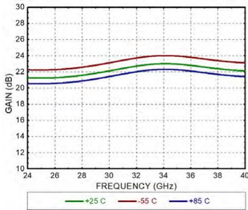
Gain
