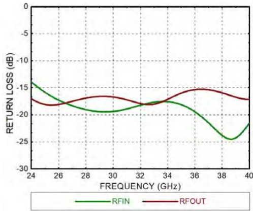
Return Loss
