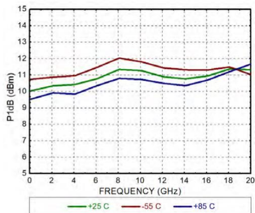
Output Power P_{1dB}
