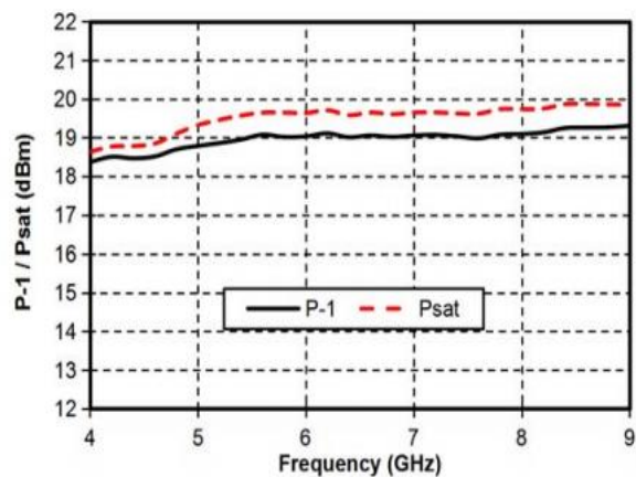
P1dB/Psat vs. Frequency
