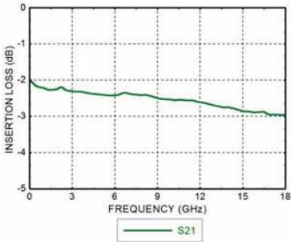
Insertion Loss
