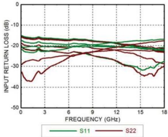
Return Loss
