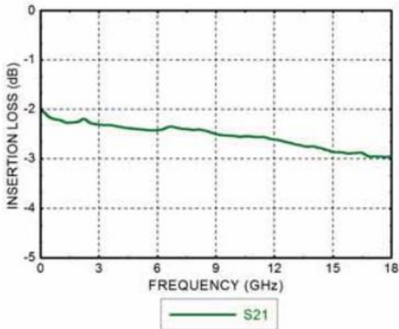
Insertion Loss
