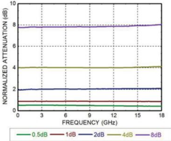
Insertion Loss
