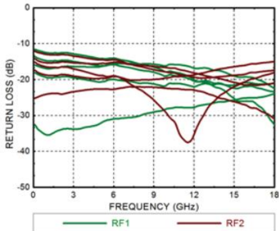
Return Loss
