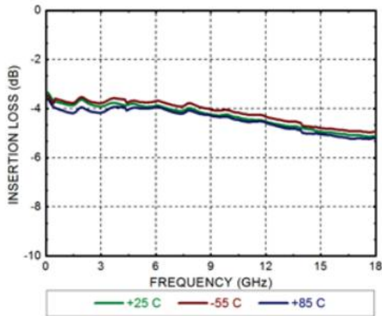
Insertion Loss
