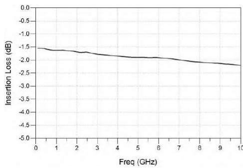
Insertion Loss
