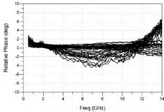
All State Attenuation Additional Phase Shift
