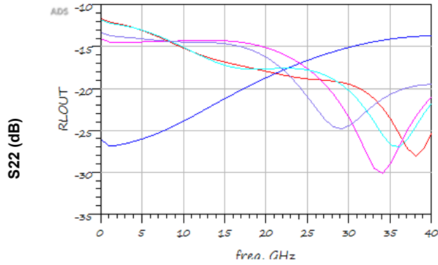
Output RL vs. Frequency
