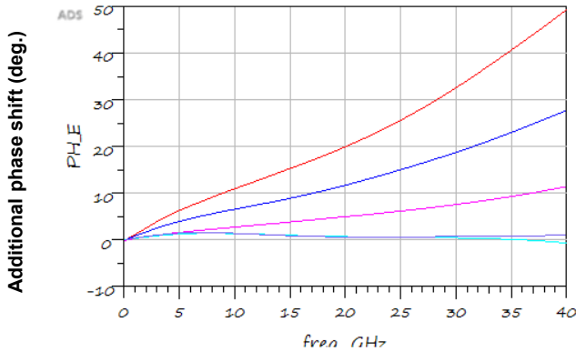
Additional phase shift vs. Frequency
