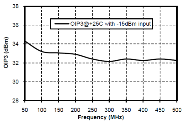
OIP3 vs. Frequency (Pin=-15dBm)
