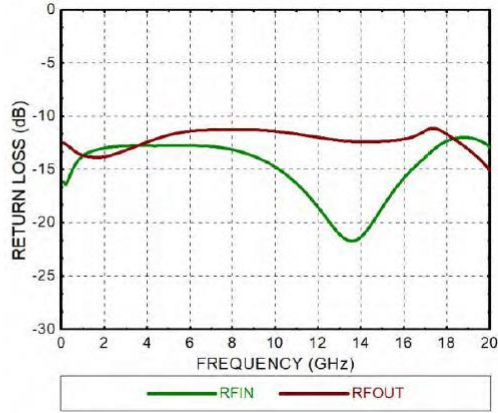
Return Loss
