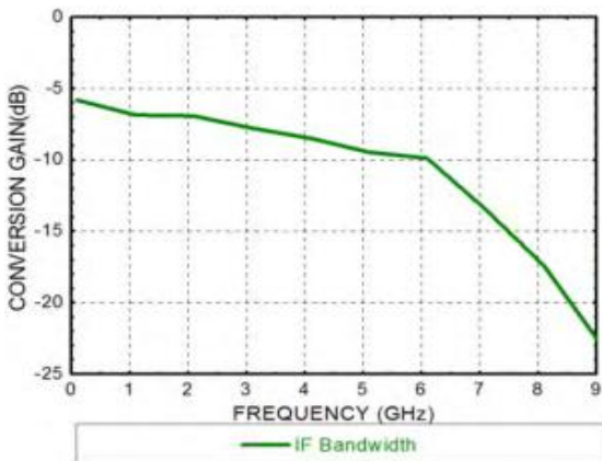
IF Bandwidth
