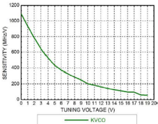
Tuning Sensitivity vs. Tuning Voltage, T=25°C
